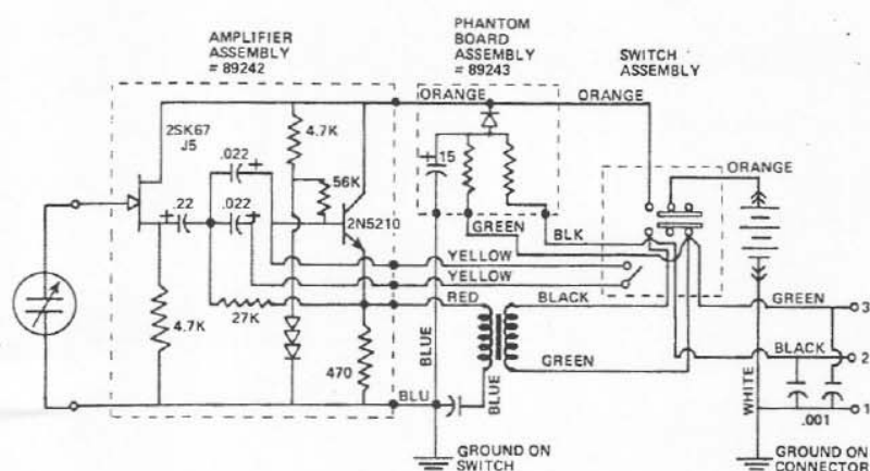
FIGURE 2 - Wiring Diagram
