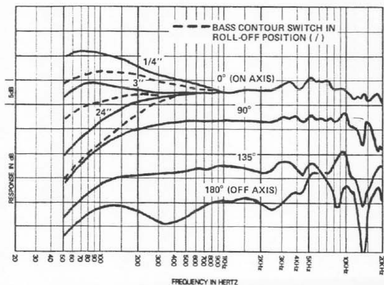
FIGURE 3 - Frequency Response
