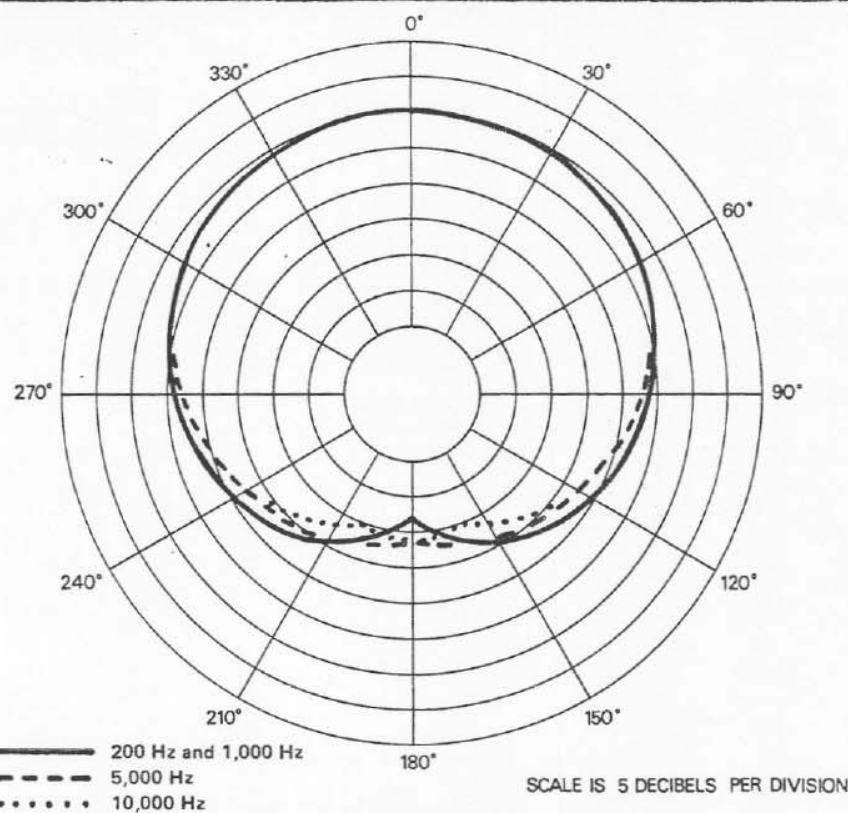
FIGURE 4 — Polar Response
